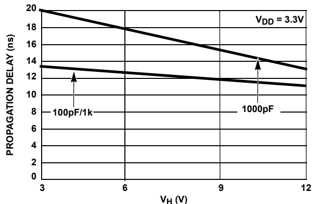
FIGURE 26. t_{pdR} vs V_H
