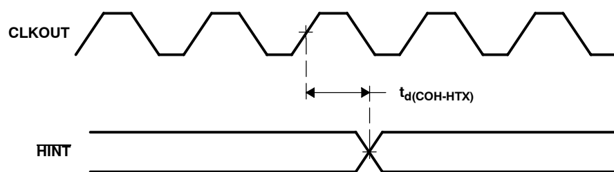
Figure 5-30. \text{HINT} Timing
