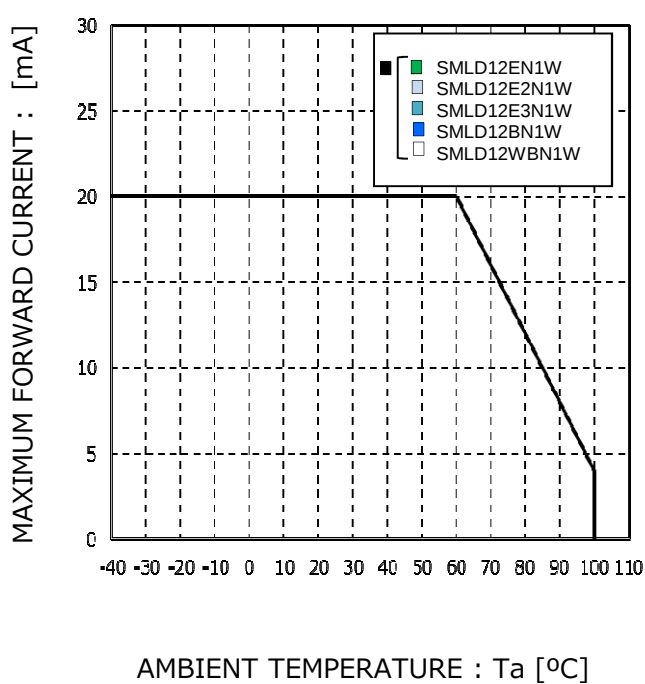
Fig.4 Derating
