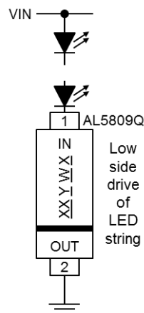
Figure 1 Low-Side LED String Drive
