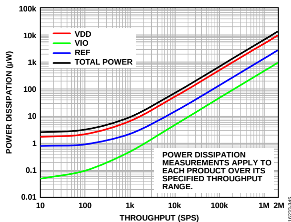
Figure 46. Power Dissipation vs. Throughput, VDD = 1.8 V, VIO = 1.8 V, VREF = 5 V, TA = 25°C
