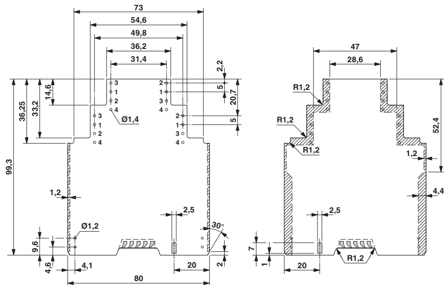
Dimensioned drawing
