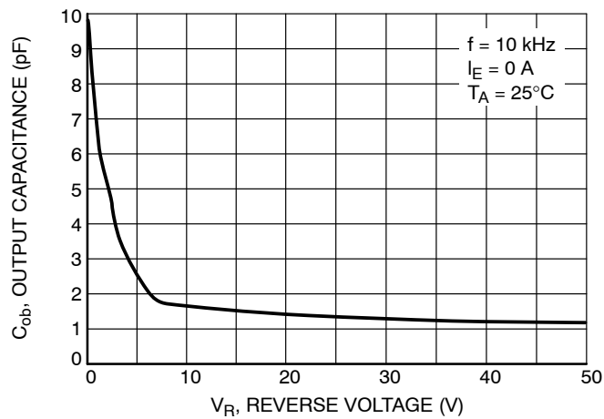
Figure 9. Output Capacitance
