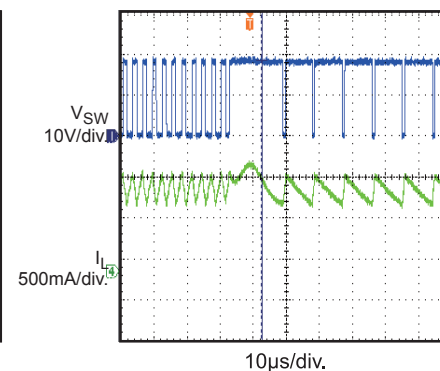
Short Protection
