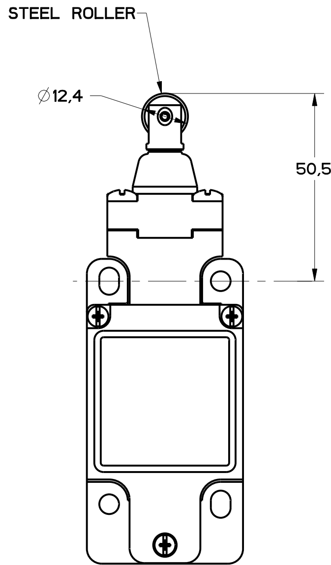
FIGURE 5 - TOP ROLLER PLUNGER HEAD OTHERWISE REFER TO FIGURE 1
