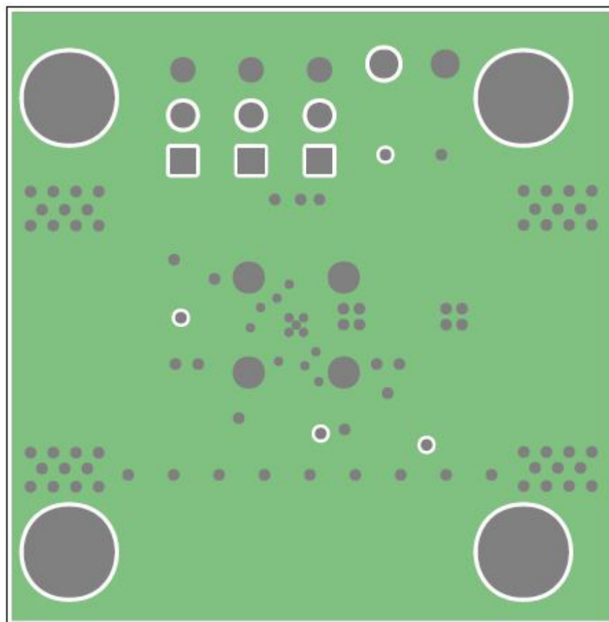
MAX2248 EV Kit—Gerber Level 3 Power
