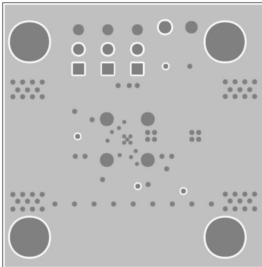
MAX2248 EV Kit—Gerber Level 2 GND
