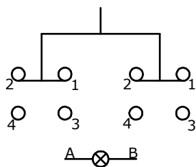
CIRCUIT: DPDT
