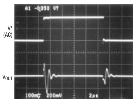
LT1218/19 • F07a
