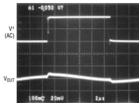
LT1218/19 • F07b
