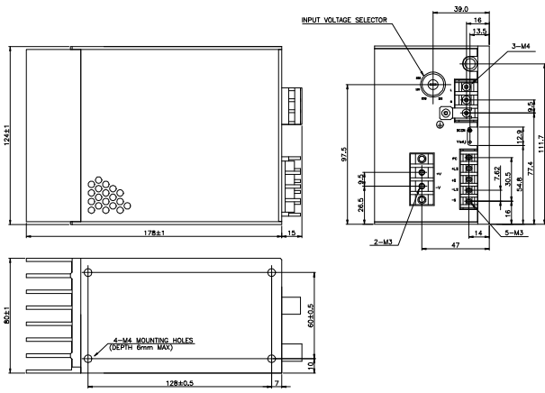
NNS30 Outline Drawing
