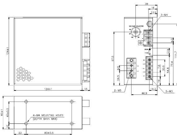
NNS15 Outline Drawing
