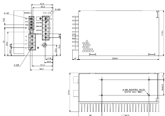
NNS50 Outline Drawing
