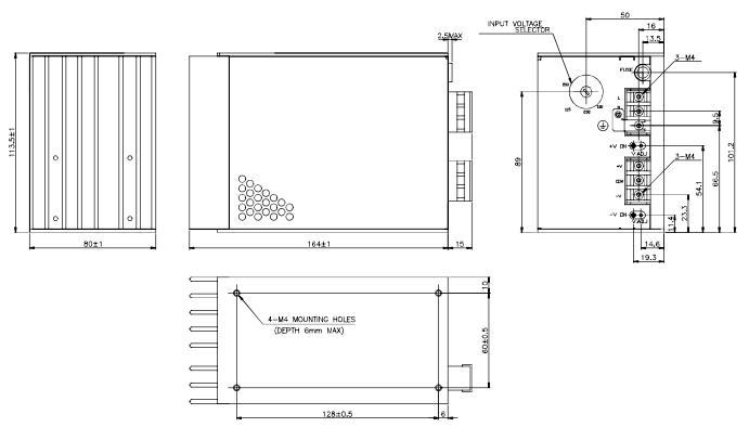
NNS50 Outline Drawing
