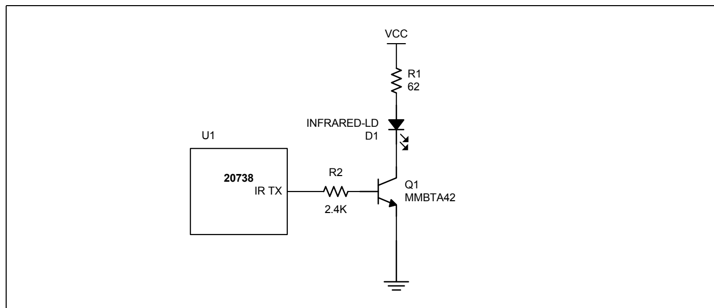
Figure 2. Infrared TX
