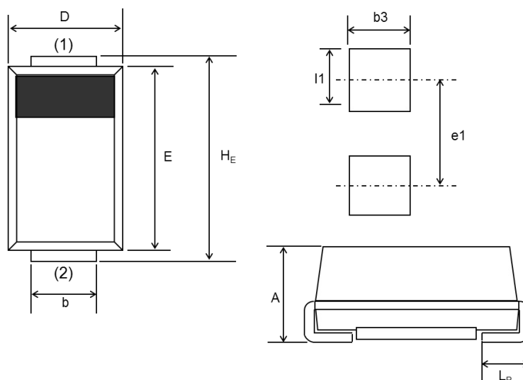
DO-214AC(SMA), (PMDS)
