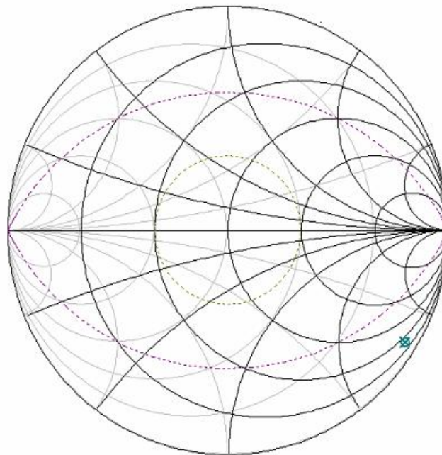
Figure 5. Device’s Input Impedance, Z = 19 - j174\Omega
