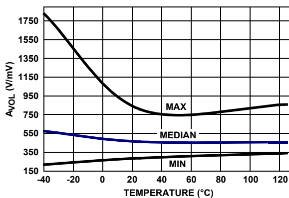
FIGURE 29. A_{VOL} vs TEMPERATURE R_L = 100k , V_+ = \pm 2.5V , V_O = -2V TO +2V
