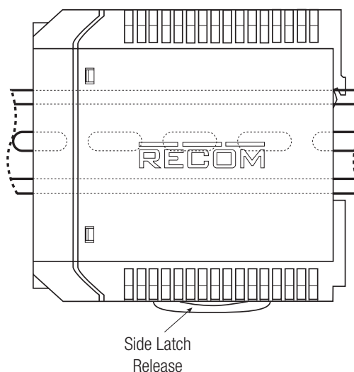
SIDE MOUNTING
