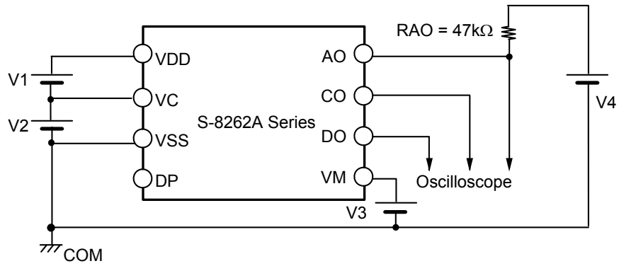
Figure 8 Test Circuit 5
