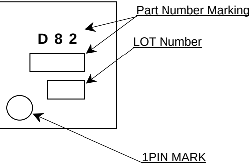
TSSOP-B8J(TOP VIEW)
