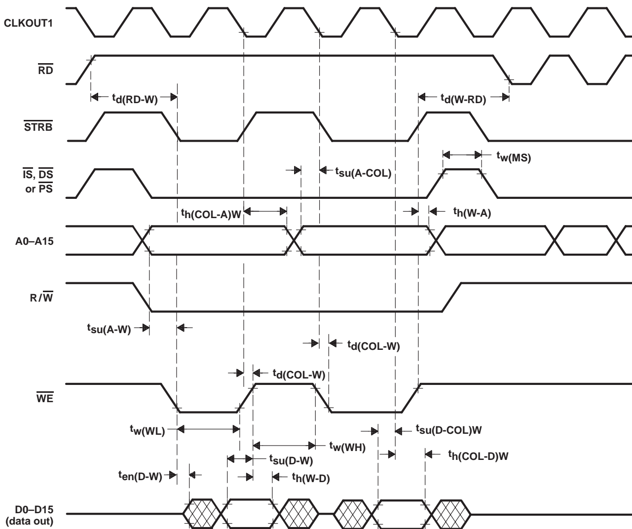
Figure 27. Memory Interface Write Timing for TMS320C209
