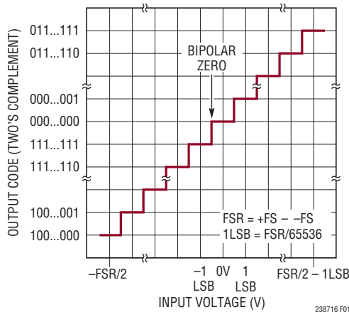
Figure 1. LTC2387-16 Transfer Function
