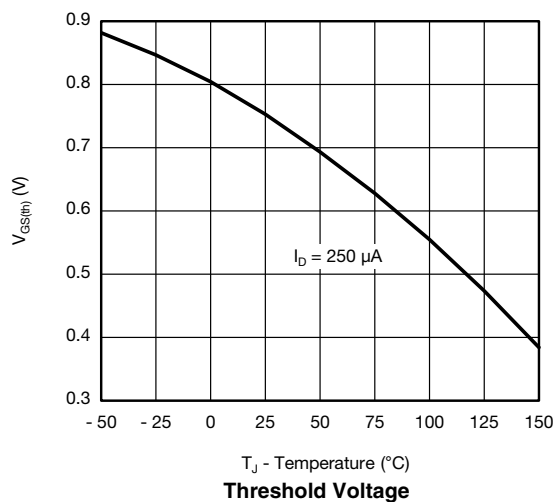
Threshold Voltage
