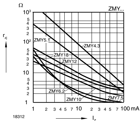
Fig. 1 - Dynamic Resistance vs. Zener Current
