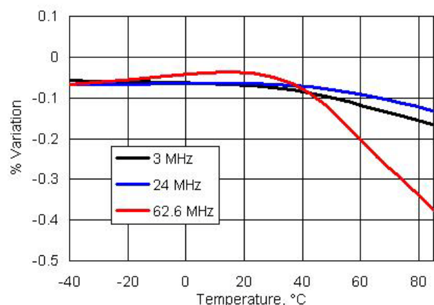
Figure 11-69. IMO Frequency Variation vs. Temperature
