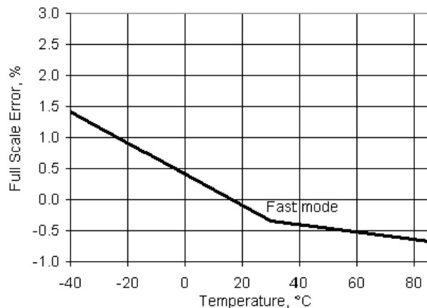
Figure 11-40. IDAC Full Scale Error vs Temperature, Range = 255 \mu A, Source Mode
