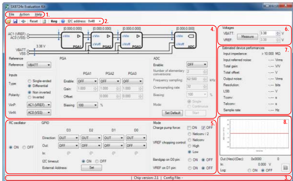
Figure 13. SX8724xEVK GUI Overview
