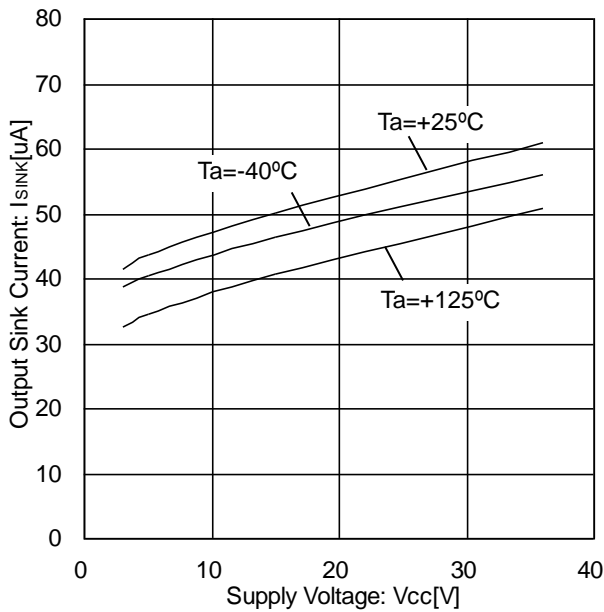
Figure 33. Output Sink Current vs Supply Voltage ( V_{OUT}=0.2\text{V} )
