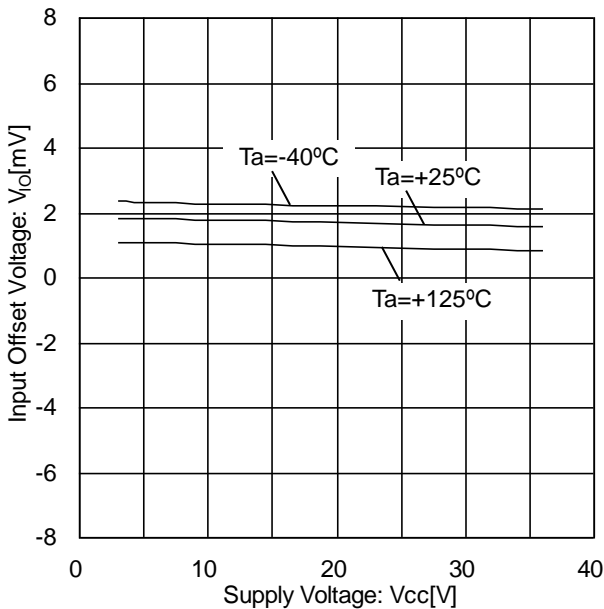
Figure 35. Input Offset Voltage vs Supply Voltage ( V_{ICM}=0\text{V} , V_{OUT}=1.4\text{V} )
