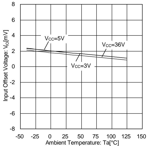
Figure 36. Input Offset Voltage vs Ambient Temperature ( V_{ICM}=0\text{V} , V_{OUT}=1.4\text{V} )
