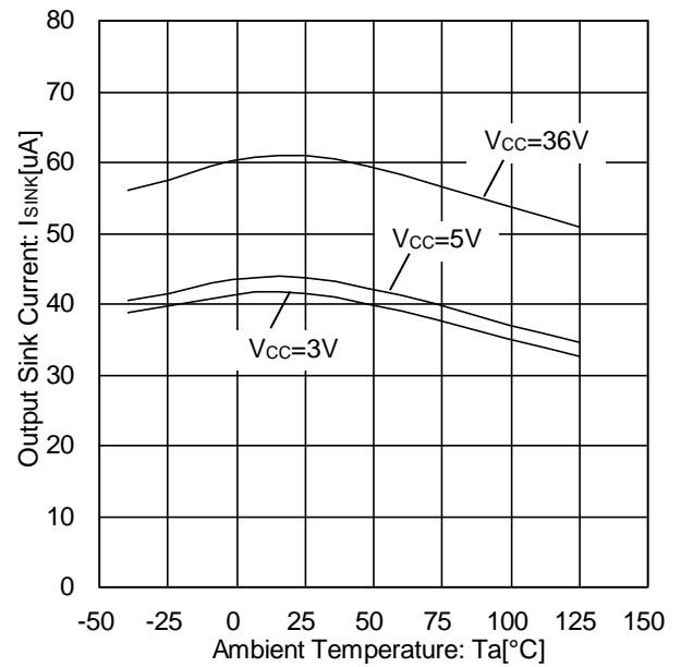
Figure 34. Output Sink Current vs Ambient Temperature ( V_{OUT}=0.2\text{V} )
