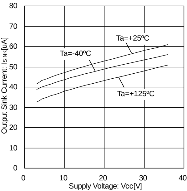
Figure 10. Output Sink Current vs Supply Voltage ( V_{OUT}=0.2V )
