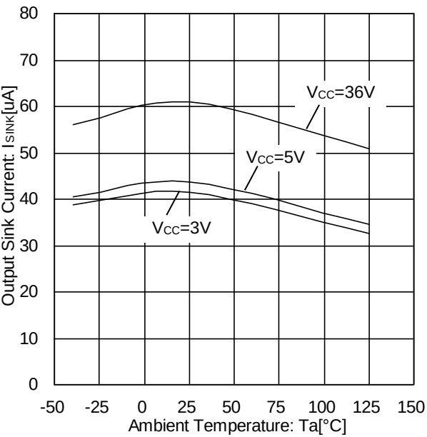
Figure 11. Output Sink Current vs Ambient Temperature ( V_{OUT}=0.2V )
