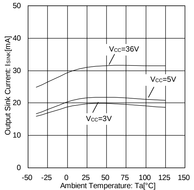
Figure 32. Output Sink Current vs Ambient Temperature ( V_{OUT}=V_{CC} )
