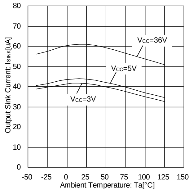
Figure 11. Output Sink Current vs Ambient Temperature ( V_{OUT}=0.2V )
