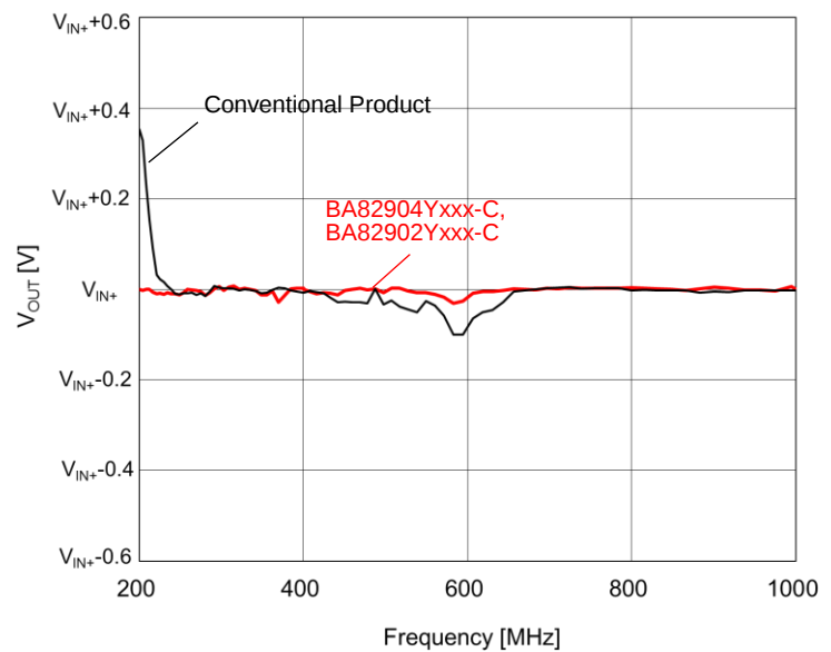
Figure 52. EMI Characteristics
