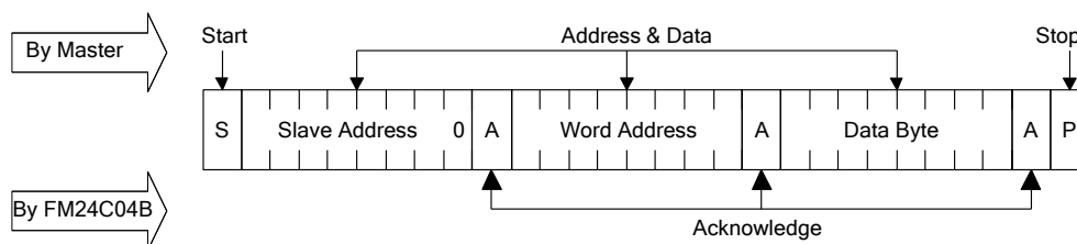
Figure 5. Byte Write
