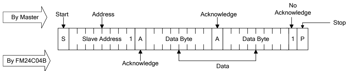
Figure 8. Sequential Read
