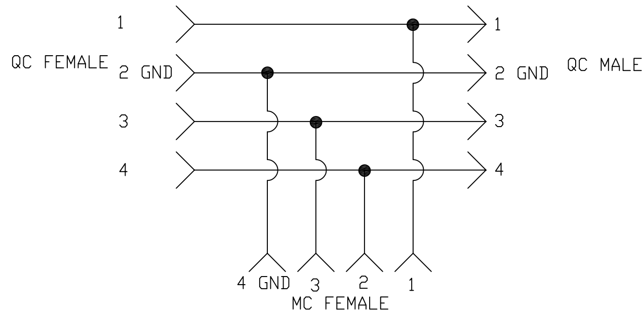
WIRE DIAGRAM
