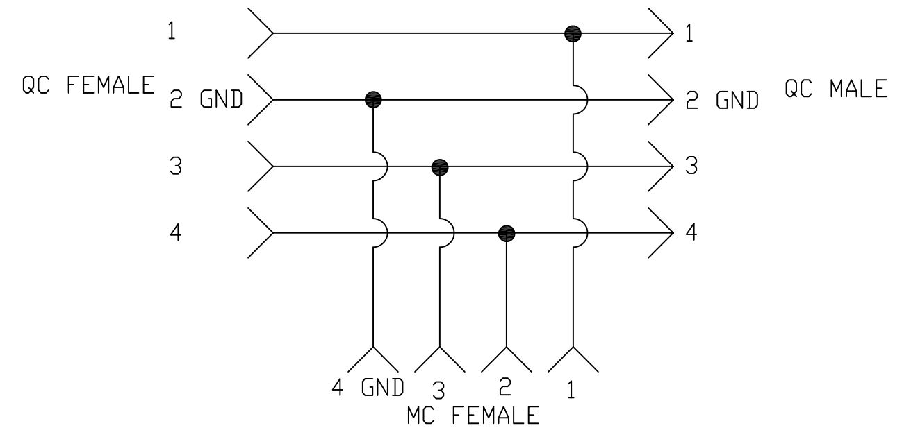
WIRE DIAGRAM
