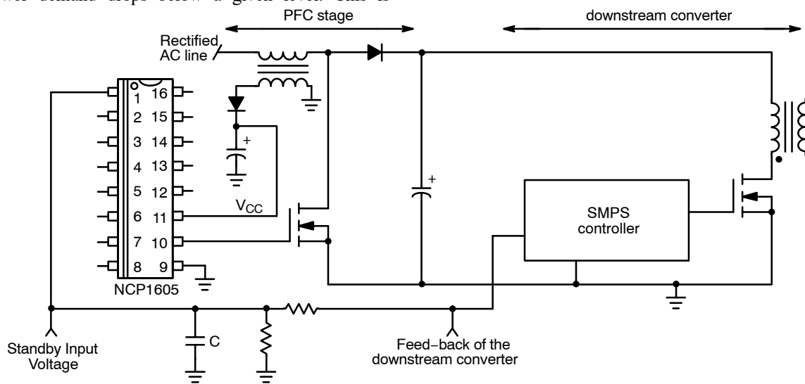
Figure 63. Signal for Standby Detection
