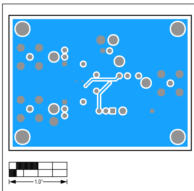
MAX4475 EV Kit—Bottom
