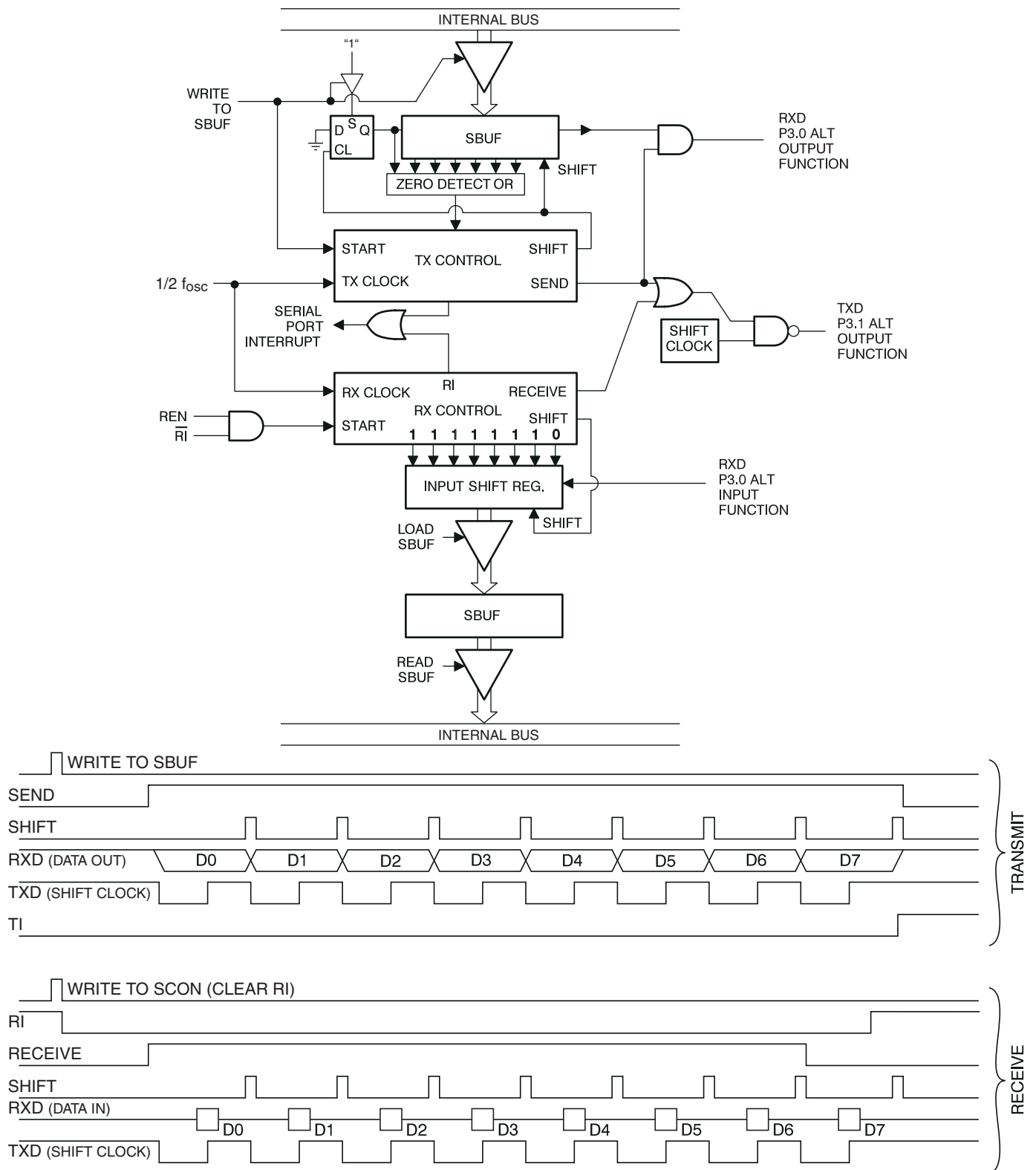
Figure 17-1. Serial Port Mode 0
