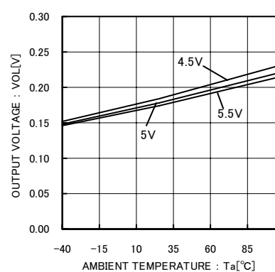
Fig.9 SEROUT low side voltage (Temperature characteristic @ ISO=4mA)
