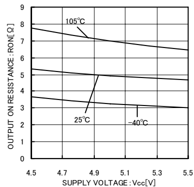
Fig.3 Output on resistance (VCC characteristic @ IDD=20mA)
