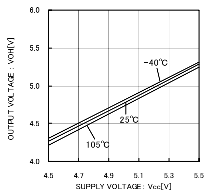
Fig.6 SEROUT high side voltage (VCC characteristic @ ISO=-5mA)
