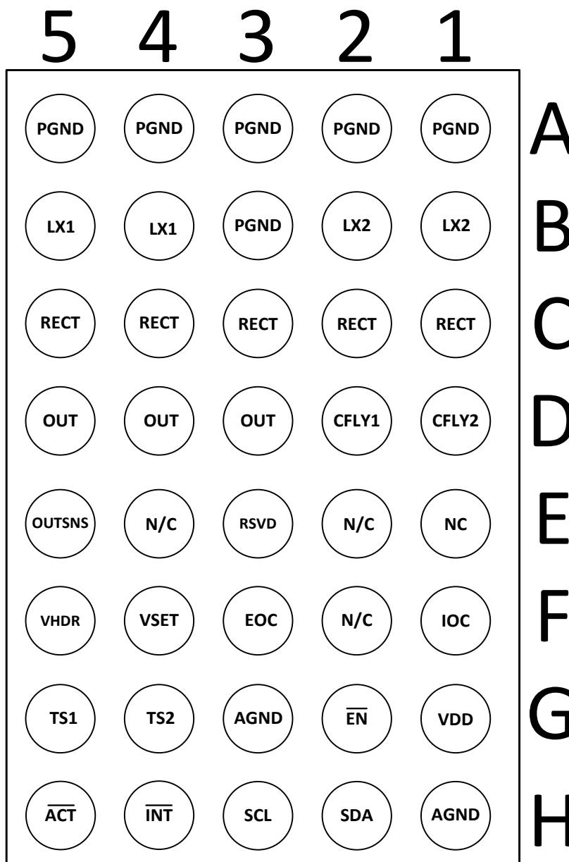
Bottom View
