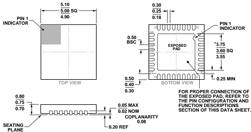
Figure 57. 32-Lead Lead Frame Chip Scale Package [LFCSP_WQ] 5 mm × 5 mm Body, Very Thin Quad (CP-32-12) Dimensions shown in millimeters
