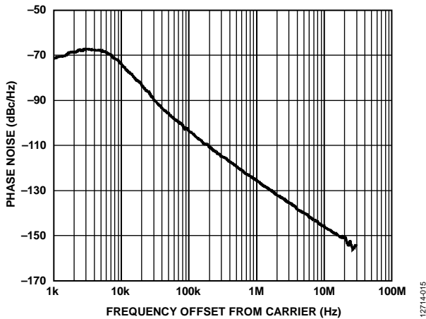
Figure 18. Closed-Loop Phase Noise, R_{F_{OUT}B} = 13.6 GHz, 2 \times VCO , VCO = 6.8 GHz, f_{PFD} = 61.44 MHz, Loop Bandwidth = 2 kHz
