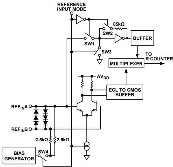
Figure 32. Reference Input Stage, Differential Mode
