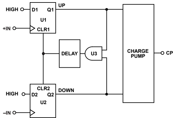
Figure 34. PFD Simplified Schematic
