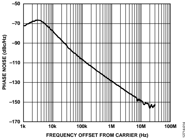
Figure 17. Closed-Loop Phase Noise, R_{F_{OUT}B} = 10 GHz, 2 \times VCO , VCO = 5.0 GHz, f_{PFD} = 61.44 MHz, Loop Bandwidth = 2 kHz
