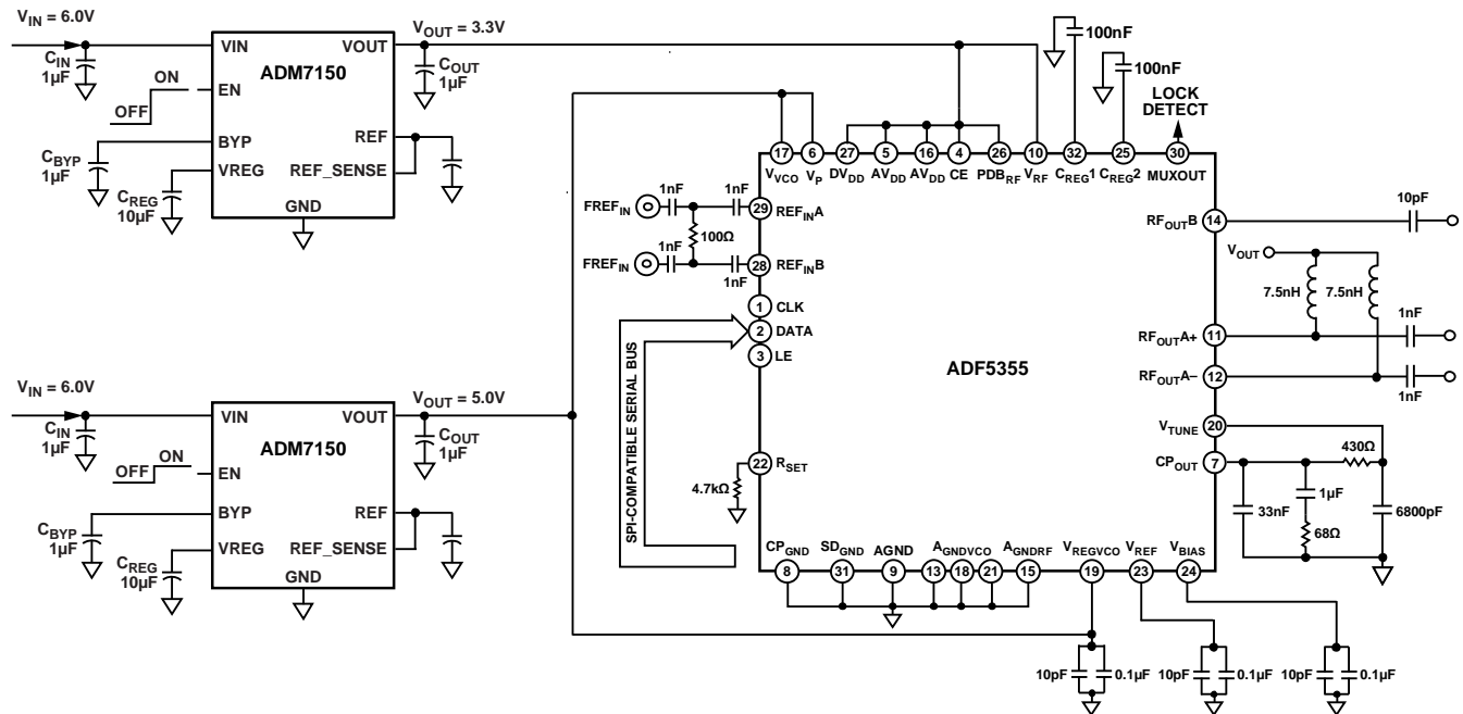
Figure 55. ADF5355 Power Supplies
