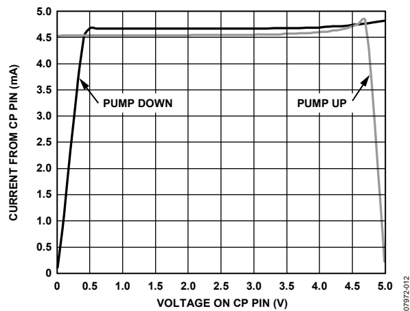
Figure 11. Charge Pump Characteristics at V_{CP} = 5.0\text{ V}
