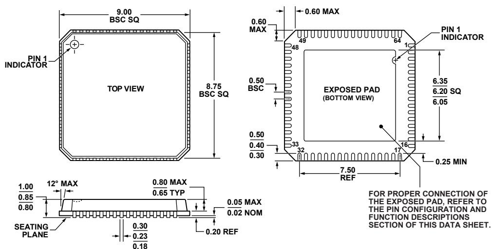
Figure 65. 64-Lead Lead Frame Chip Scale Package [LFCSP_VQ] 9 mm × 9 mm Body, Very Thin Quad (CP-64-4)
