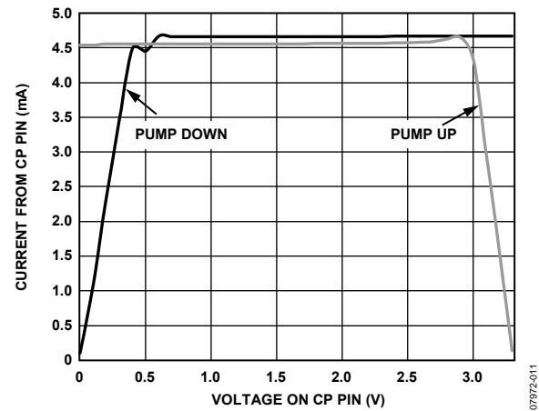
Figure 10. Charge Pump Characteristics at V_{CP} = 3.3\text{ V}
