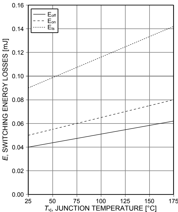
Figure 15. Typical switching energy losses as a function of junction temperature (inductive load, V_{CE}=400\text{V} , V_{GE}=15/0\text{V} , I_c=2,5\text{A} , r_G=68\Omega , Dynamic test circuit in Figure E)
