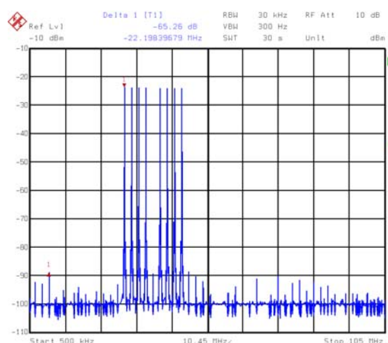
FIGURE 10. EIGHT TONES (CREST FACTOR=8.9) AT 37MHz, 210MSPS CLOCK, 2.1MHz SPACING (65dBc - NYQUIST)
