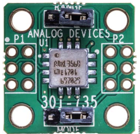
Figure 1. EVAL-ADXL356BZ/EVAL-ADXL356CZ
