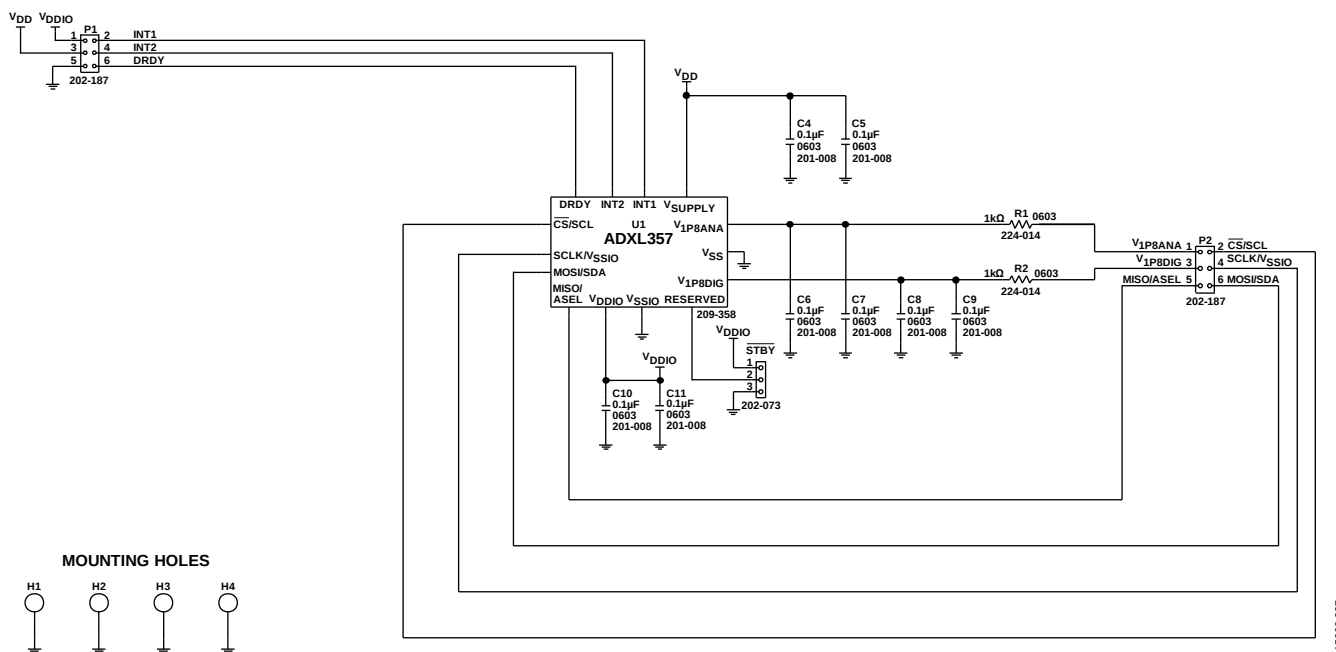
Figure 8. EVAL-ADXL357Z Schematic
