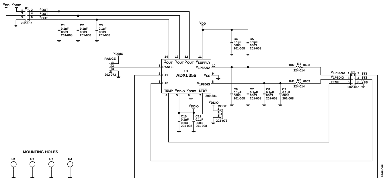
Figure 7. EVAL-ADXL356BZ/EVAL-ADXL356CZ Schematic
