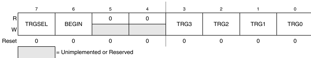
Figure 18-8. Debug Trigger Register (DBGTR)
