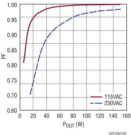
Figure 3. Power Factor vs Load
