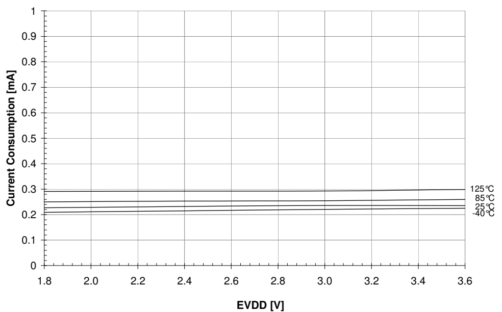
Figure 36-13. Combined Supply Current of Bandgap Source and Voltage Regulator
