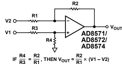
IF \frac{R4}{R3} = \frac{R2}{R1} , THEN V_{OUT} = \frac{R2}{R1} \times (V1 - V2) Figure 64. Using the AD857x as a Difference Amplifier
