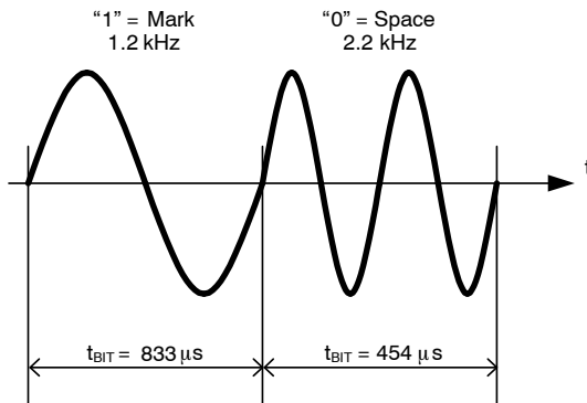
Figure 6. Modulation Timing
